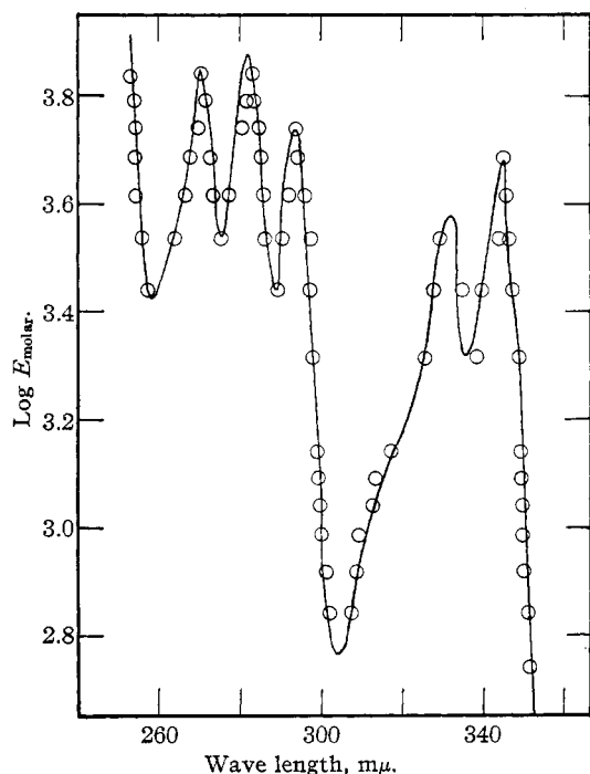
Fig. 1.—Ultraviolet absorption curve of equilenin, showing the logarithm of the extinction coefficient at various wave lengths. The solid line represents the curve for natural equilenin, the circles the values for synthetic d -equilenin.
