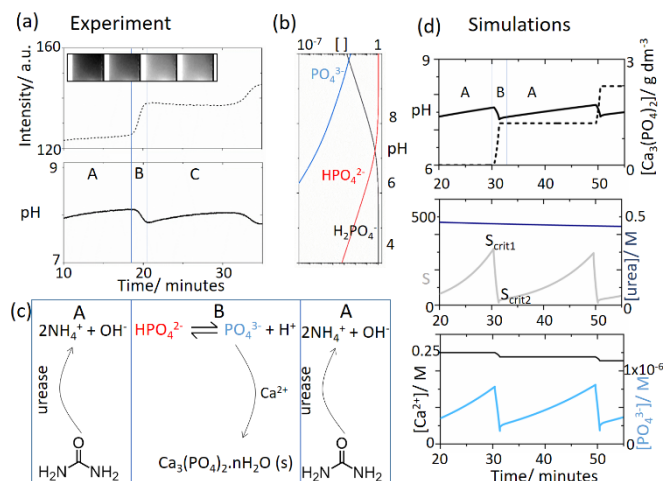
Figure 3. Periodic precipitation split into time zones A and B and (a) intensity and pH from the experiments in Figure 1(c). (b) Distribution of phosphate species as a function of pH calculated from the various equilibria, (c) basic mechanism of pH increase in A and pH decrease in B, (d) simulations showing pH and [ATCP] in time, urea and supersaturation S , and calcium and phosphate ions for initial concentrations: [urea] = 0.5 M, [HCl] = 5 mM, [CaCl 2 ] = 0.25 M, [urease] = 30 u/ml, [H 2 PO 4 - ] = 0.05 M.
