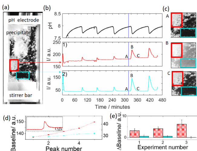
Figure 2. Periodic nucleation and aggregation of calcium phosphate in a cuvette with low stirring rate (200 rpm) where [urea] = 0.5 M, [HCl] = 5 mM, [CaCl 2 ] = 0.25 M, [urease] = 30 u/ml, [H 2 PO 4 - ] = 0.05 M. (a) image of the cuvette where the white agglomerates of precipitate are deposited on the walls and pH electrode. (b) Time series of pH, 1) average intensity of images of wall-coating aggregates in the red box and 2) average intensity in images of the bulk solution in the blue box. The blue line indicates the time point at which the image on the left was taken. (c): images of part of the cuvette at time points indicated A, B and C. (d) Baseline intensity after a peak from an area in the cuvette with aggregate (red) and without aggregate (blue) for experiment in (a). Inset shows peak and change in baseline intensity. (e) Average change in baseline intensity from areas with aggregate (red) and areas without aggregate (blue) for three repeats of the experiment. Error bars indicate standard deviation calculated from multiple sample areas.
