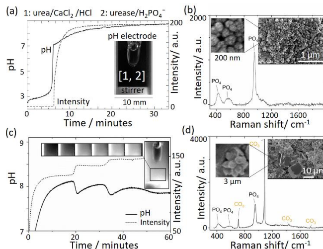
Figure 1. Precipitation of calcium phosphate in a cuvette with high stirring rate (1000 rpm). (a) Changes in pH and intensity of grayscale images with initial concentrations of [urea] = 0.08 M, [CaCl 2 ] = 4 mM, [HCl] = 3 mM, [urease] = 20 u/ml, [H 2 PO 4 - ] = 0.034 M. (b) Raman spectrum with PO 4 peaks at ~420, 586 and 952 cm -1 and SEM of precipitates formed with concentrations in (a). (c) Periodic, stepwise precipitation and pH oscillations with [urea] = 0.5 M, [CaCl 2 ] = 0.25 M, [HCl] = 5 mM, [urease] = 20 u/ml, [H 2 PO 4 - ] = 0.034 M. (d) Raman spectrum from precipitate taken during the reaction with concentrations in (d) except [urease] = 30 u/ml and [H 2 PO 4 - ] = 0.05 M with broad PO 4 peaks at ~420, 586 and 952 cm -1 and CO 3 peaks at 712, 1086, 1437 and 1747 cm -1 . Inset: SEM of precipitates.
