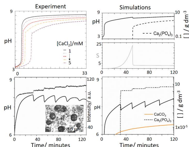
Figure 4. Comparison of reaction profiles in experiments and simulations for different reaction conditions (a) pH profile in experiments with low calcium chloride concentration where [urease] = 20 u/ml, [H 2 PO 4 - ] = 0.034 M, [urea] = 0.08 M, [HCl] = 3 mM, and [CaCl 2 ] = 1 – 5 mM, (b) simulations with same conditions as in Figure 3(d) but reduced calcium chloride [CaCl 2 ] = 0.03 M. (c) oscillations with [urea] = 0.5 M, [CaCl 2 ] = 0.25 M, [HCl] = 5 mM, [urease] = 30 u/ml, [H 2 PO 4 - ] = 0.05 M. Inset shows optical microscope image of a sample of the reaction after oscillations with small scale precipitates (calcium phosphate) and larger structures (calcite) (d) Simulations showing production of calcium phosphate (dashed) and calcite (orange) with [urea] = 0.5 M, [CaCl 2 ] = 0.25 M, [HCl] = 5 mM, [urease] = 30 u/ml, [H 2 PO 4 - ] = 0.05 M.
