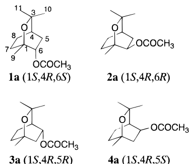
Figure 1. Structures of 2- and 3-acetoxy-1,8-cineoles. The common names and the systematic names are as follows: 1a , trans -2-acetoxy-1,8-cineole ( trans -1,3,3-trimethyl-2-oxabicyclo[2.2.2]oct-6-yl acetate); 2a , cis -2-acetoxy-1,8-cineole ( cis -1,3,3-trimethyl-2-oxabicyclo[2.2.2]oct-6-yl acetate); 3a , trans -3-acetoxy-1,8-cineole ( trans -1,3,3-trimethyl-2-oxabicyclo[2.2.2]oct-5-yl acetate); 4a , cis -3-acetoxy-1,8-cineole ( cis -1,3,3-trimethyl-2-oxabicyclo[2.2.2]oct-5-yl acetate). Each acetoxy-1,8-cineole has two optical isomers, and one of them is shown here. The absolute configuration is indicated in parentheses. The numbering corresponds to the systematic name.
