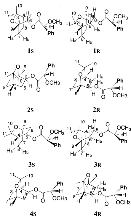
Figure 2. Structures of (S)-(+)-O-methylmandelate esters of 2- and 3-hydroxy-1,8-cineoles. For the numbering, the legend of Figure 1 should be referred to. Absolute configurations of each compound are as follows: 1s (1S,4R,6S); 1R (1R,4S,6R), 2s (1R,4S,6S); 2R (1S,4R,6R); 3s (1R,4S,5S); 3R (1S,4R,5R); 4s (1S,4R,5S); 4R (1R,4S,5R).
