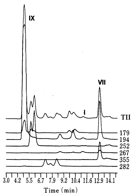
Fig. 5. Mass Chromatogram of O-TMS Derivatives of Oxidation Products of IX
