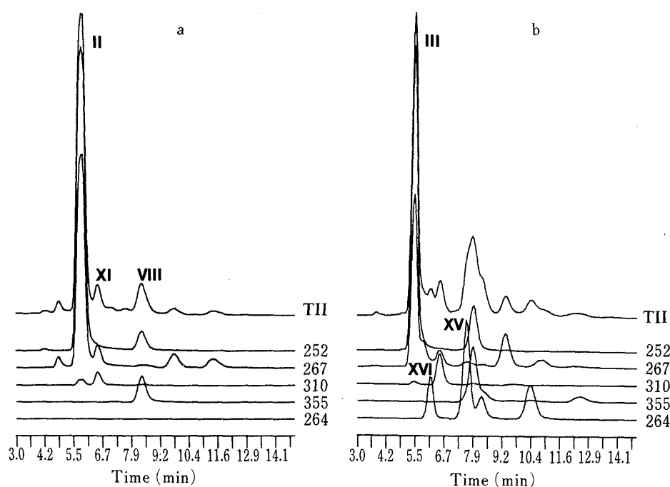
Fig. 3. Mass Chromatograms of O-TMS Derivatives of Oxidation Products of (a) II and (b) III
