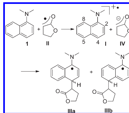
Scheme 6. Electrophilic Aromatic Substitution with Electrophilic Radical II and Naphthylamine Derivative 1 Involving Single Electron Transfer As Outlined in Scheme 4
