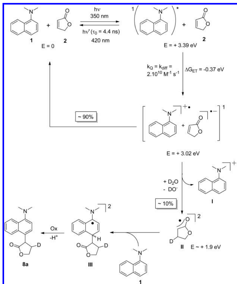
Scheme 3. Mechanism of the Photochemical Electron Transfer Mediated Addition of Naphthylamine Derivative 1 to Furanone 2
