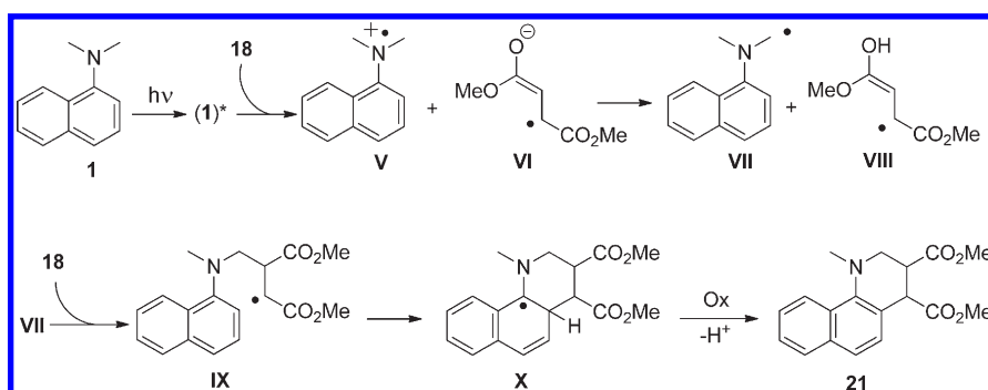
Scheme 10. Mechanism of Formation of Minor Product 21
