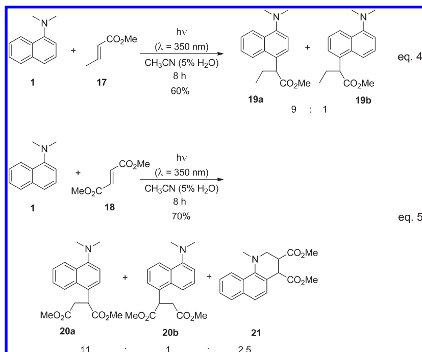
Scheme 9. Photochemical Addition of Naphthylamine Derivative 1 to Acyclic \alpha,\beta -Unsaturated Esters 17 and 18
