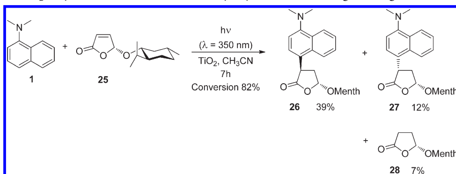
Scheme 12. Addition of Naphthylamine Derivative 1 to Menthylloxifuranone 25 Using Heterogeneous Photocatalysis with \text{TiO}_2 a
