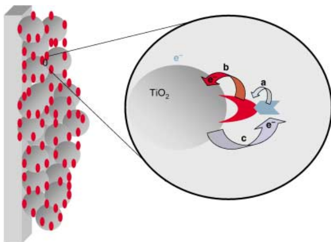
Scheme 1. Schematic representation of electron-transfer (ET) processes in dye-sensitised solar cells showing photogeneration of the dye excited state: a) electron transfer from the secondary electron donor moiety, b) electron injection into the semiconductor and c) the wasteful charge-recombination pathway of the injected electron with the oxidised dye molecules.
