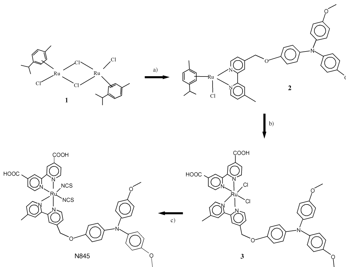
Scheme 2. Schematic of pathways for the synthesis of the N845 dye: a) 4-[4-( N,N -di- p -anisylamino)phenoxyethyl]-2,2'-bpy, b) DMF, N 2 , 4,4'-dicarboxy-2,2'-bpy, c) NH 4 NCS, N 2 , DMF.
