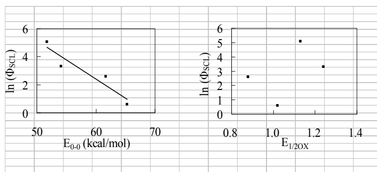
Figure 1. The correlation diagrams. a: \ln(\Phi_{SCL}) vs E_{0-0} (kcal/mol) and b: \ln(\Phi_{SCL}) vs E_{1/2OX}
