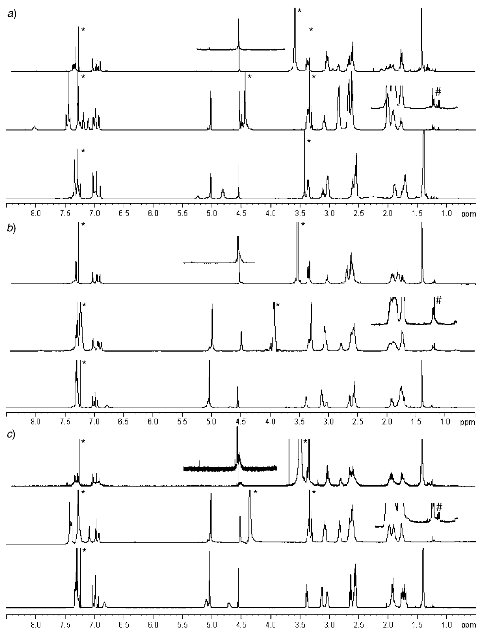
Fig. 1. ^1\text{H} -NMR Spectra of a) 7a , b) 7b , and c) 9b and their respective selectively deprotected counterparts (see text) to show the degrees to which the deprotections can be achieved. *: Solvent signals, #: grease signals.
