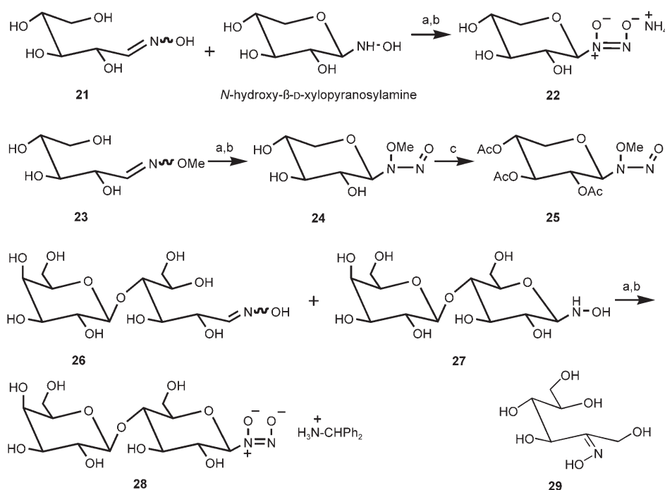
Scheme 2. Reactions of xylose, lactose, and fructose oximes with \text{NO}^+ . a) \text{HCl}/\text{H}_2\text{O} + \text{NaNO}_2 . b) \text{Ph}_2\text{CH}-\text{NH}_2 . c) \text{Ac}_2\text{O}/\text{pyridine} .
