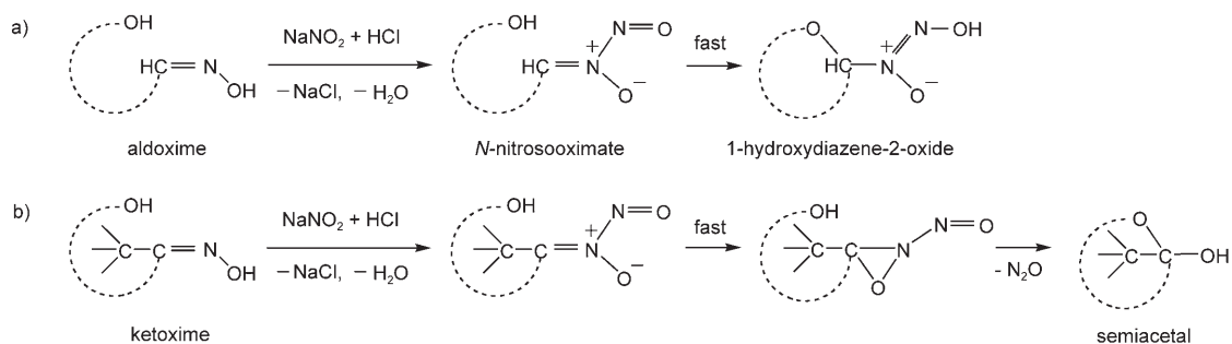
Scheme 3. Proposed nitrosation mechanisms for \omega -hydroxyaldoximes and \omega -hydroxyketoximes.
