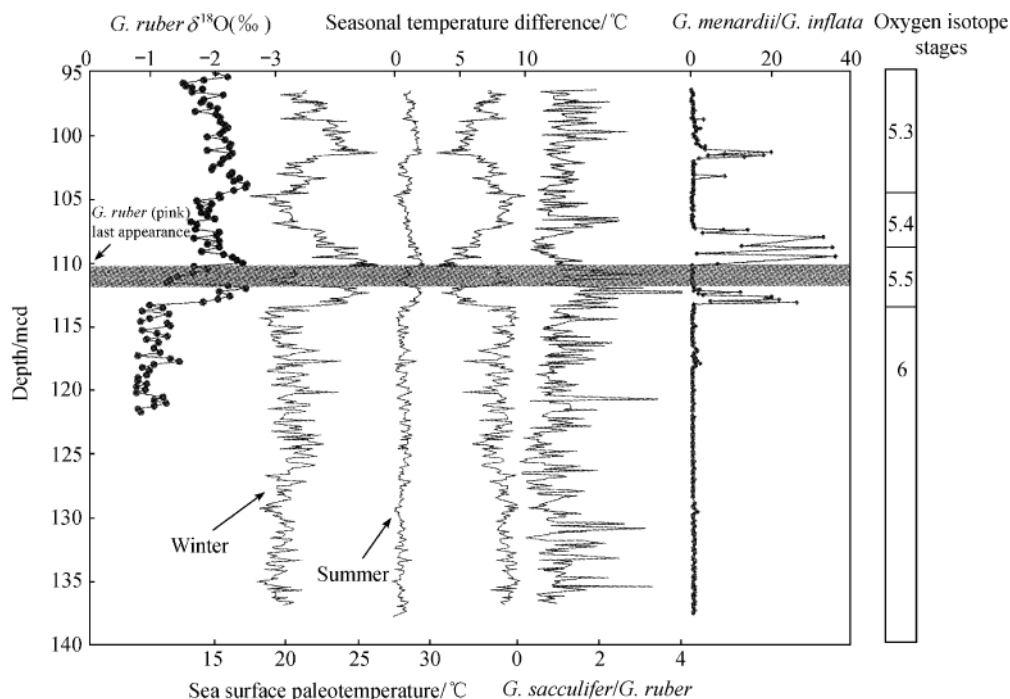
Fig. 1. Downcore variations of SST based on transfer function, oxygen isotope, G. sacculifer/G. ruber ratio and G. menardii/G. inflata ratio from MIS 5.3 to MIS 6 at ODP Site 1144, northern South China Sea (Shaded bar indicates the abrupt cooling event within MIS 5.5).
