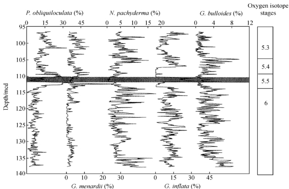
Fig. 2. Downcore variations of some planktonic foraminiferal species from MIS 5.3 to MIS 6 at ODP Site 1144, northern South China Sea (Shaded bar indicates the abrupt cooling event within MIS 5.5).
