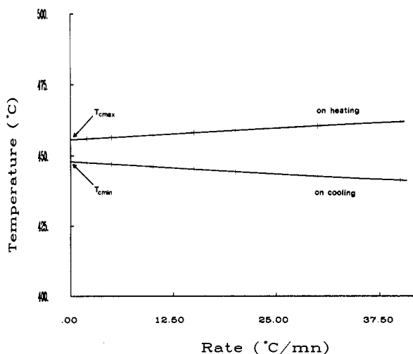
Figure 1. T_{peak} as a function of the rate R on cooling and heating in the DSC analysis. T_{cmax} = 456^\circ C , T_{cmin} = 448^\circ C .
