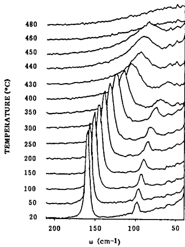
Figure 4. Temperature dependence of the Raman spectra of AlF 3 .
