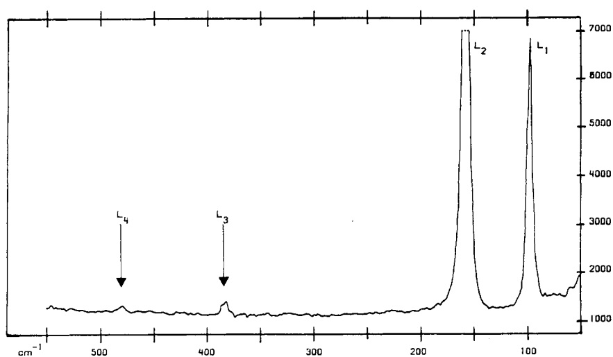
Figure 3. Room temperature Raman spectrum of \text{AlF}_3 .
