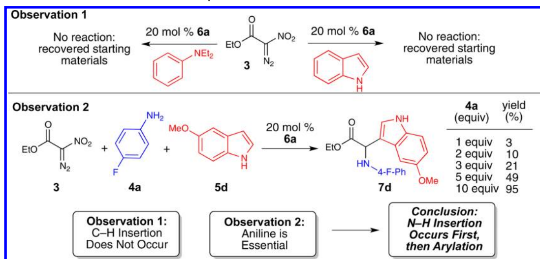
Scheme 3. Initial Clues into the Reaction Pathway
