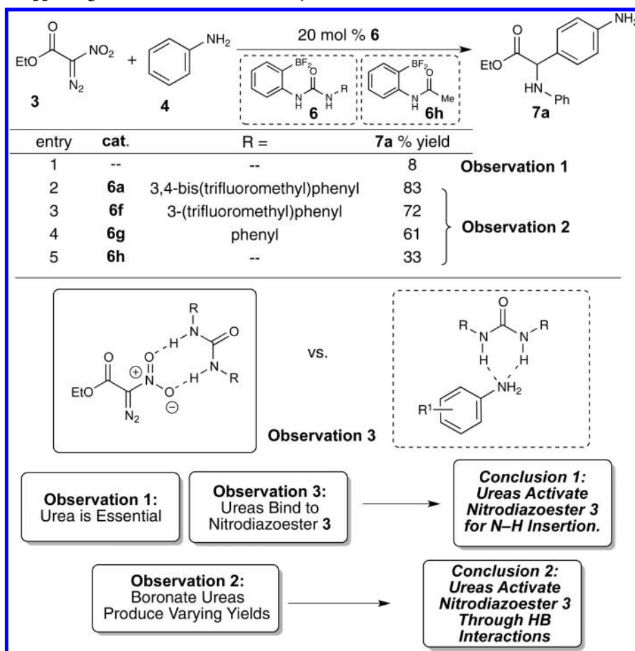
Scheme 4. Evidence Supporting the Role of the Urea Catalyst
