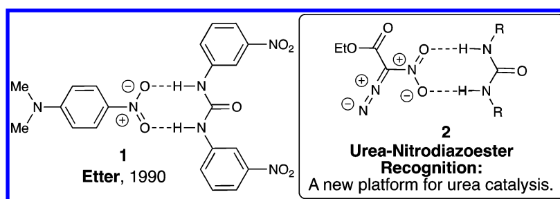
Figure 1. Urea–nitro group recognition as a platform for catalysis.
