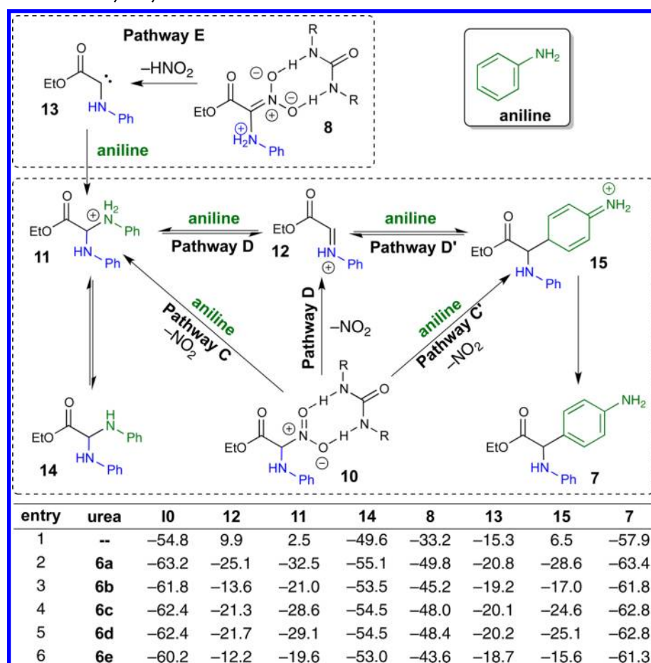
Scheme 7. Possible Routes for Aryl Glycine Formation a
