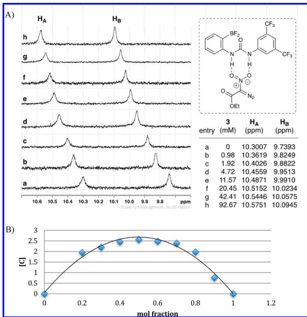
Figure 2. Urea-nitrodiazoester binding titration studied by 1 H NMR spectroscopy in acetone- d 6 at 298.0 K. (A) Selected titration spectra with corresponding concentrations and NMR chemical shifts. Titration data (0–262 equiv of guest 3) were fit to a 1:1 binding model. See the Supporting Information for experimental details. (B) Job plot analysis suggesting 1:1 binding stoichiometry.
