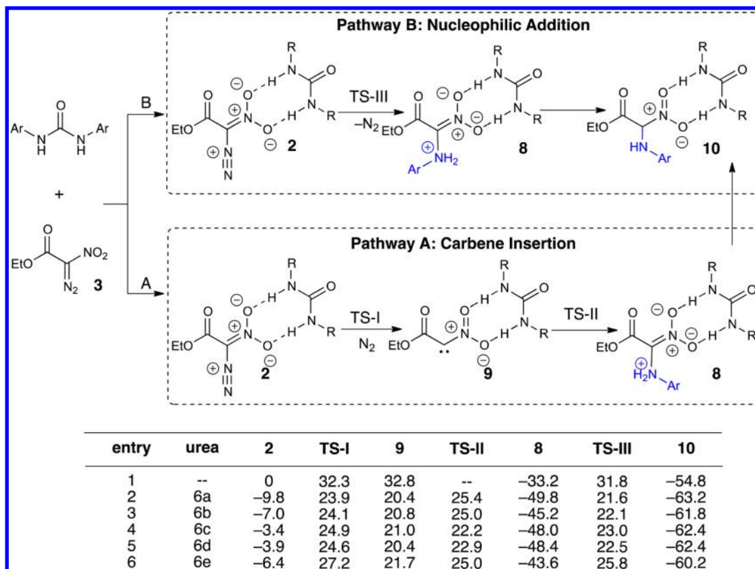
Scheme 5. Plausible Pathways of Urea-Catalyzed N–H Insertion/Multicomponent Coupling of Nitrodiazoesters a
