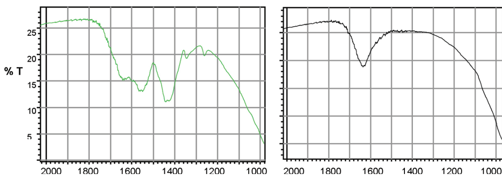
Figure 9. Transmission FTIR spectra of pellets of platinized TiO 2 (5% Pt) prepared by the photodeposition method before heat treatment (left) and after heating at 500 °C in vacuo for 3 h (right). Spectral window 2000–1000 cm -1 .
