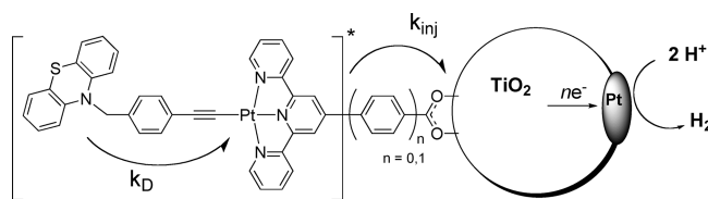
Figure 4. Schematic representation of D-C dyads 3 ( n = 1 ) and 4 ( n = 0 ) as sensitizers for the photogeneration of hydrogen. k_D is the rate constant for reductive quenching of the chromophore by the phenothiazine moiety.
