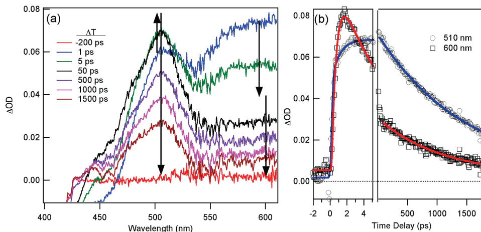
Figure 8. (a) Transient absorption spectra of dyad 6 in acetonitrile, collected at various intervals after excitation. (b) Kinetics of the photoinduced absorption changes at 510 and 600 nm showing the rapid loss of absorption at 600 nm and the long-time decay of both signals in 1–1.5 ns. The excitation wavelength was 400 nm.
