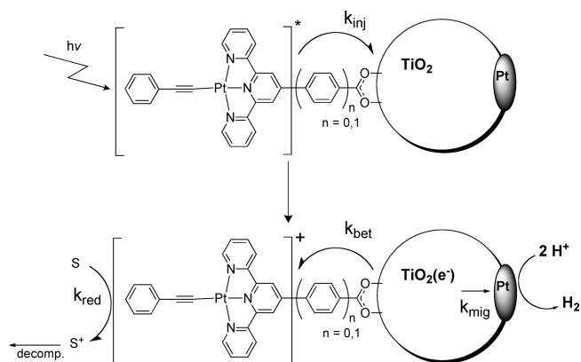
Figure 2. Schematic representation of a system for the photogeneration of hydrogen, using platinum terpyridyl acetylides 1 ( n = 1 ) and 2 ( n = 0 ) to sensitize platinized TiO 2 . The processes of charge injection, back electron transfer, charge migration through the particle, and reduction by the sacrificial donor have rate constants denoted as k_{inj} , k_{bet} , k_{mig} , and k_{red} , respectively.
