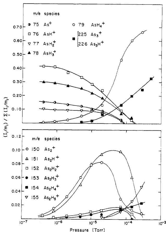
Figure 1. Variation of ion abundance with pressure for \text{AsH}_3 at 70 eV. The tertiary ions \text{As}_3^+ and \text{As}_3\text{H}^+ were poorly resolved in single-resonance spectra at high pressures. Their intensities are reported as an approximate sum.
