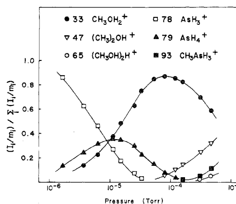
Figure 5. Variation of ion abundance with pressure for a 3:1 mixture of \text{AsH}_3 and \text{CH}_3\text{OH} at 11 eV.
