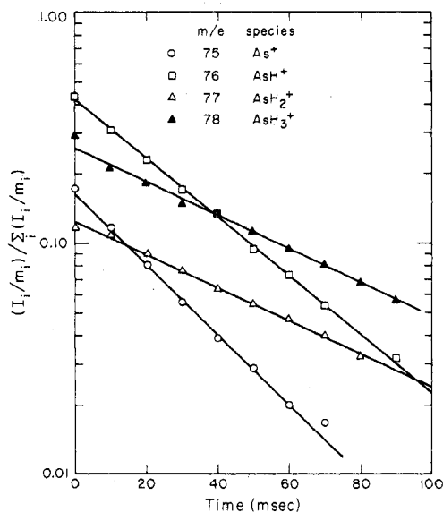
Figure 3. Variation of \log (relative ion abundance) with time for the four primary ions in \text{AsH}_3 at 70 eV and 1.9 \times 10^{-6} Torr. The slope of the line for each ion yields the total disappearance rate constant for that species.
