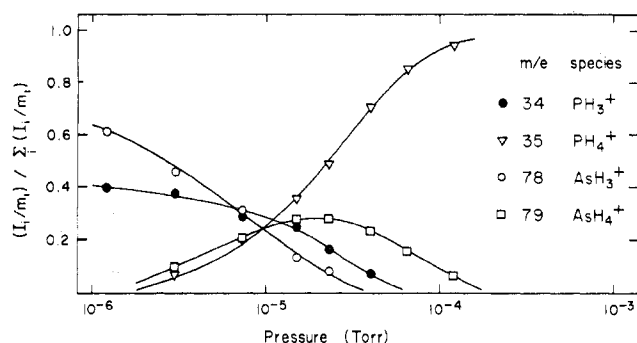
Figure 4. Variation of ion abundance with pressure for a 1.6:1 mixture of \text{AsH}_3 and \text{PH}_3 at 11 eV.
