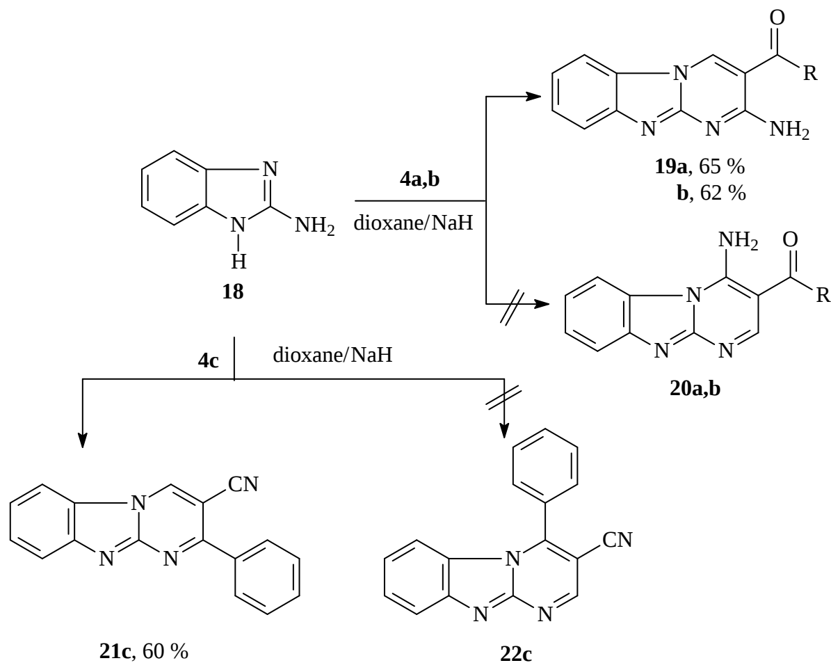
Scheme 4
