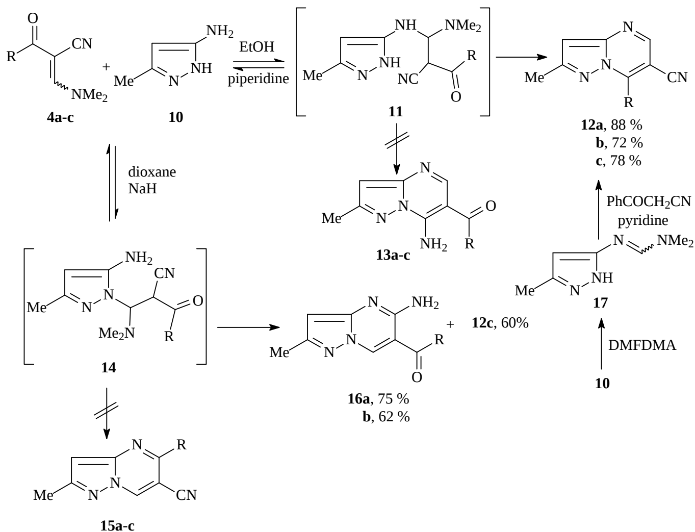
Scheme 3
