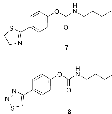
Fig. 3. The lead structures SPB01403 ( 7 ) and SEW01169 ( 8 ).
