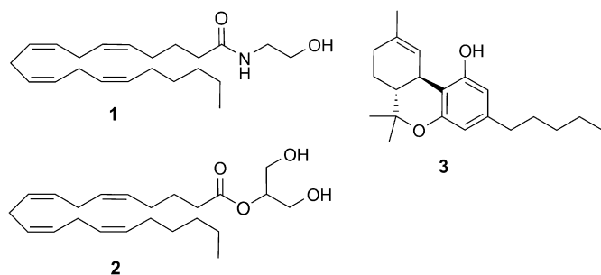
Fig. 1. Structures of N -arachidonylethanolamine (AEA, 1 ), 2-arachidonoylglycerol (2-AG, 2 ), and \Delta^9 -tetrahydrocannabinol ( \Delta^9 -THC, 3 ).
