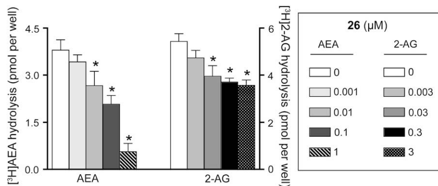
Fig. 6. Effect of 26 upon the hydrolysis of 0.10 μM [ ^3\text{H} ]AEA and [ ^3\text{H} ]2-AG by RBL2H3 cells. Data are means and s.e.m., n = 5 (AEA) or n = 4 (2-AG). * p < 0.05 vs corresponding control, Dunnett's multiple comparison test following significant one-way ANOVA for repeated measures. Expressing the data as % of control for AEA gave values of 92 \pm 7 , 70 \pm 8 , 55 \pm 6 and 15 \pm 7 for 0.001, 0.01, 0.1 and 1 μM 26 , respectively (means \pm s.e.m.). These values give an \text{IC}_{50} value of 0.082 μM (constraining "top" and "bottom" values of the analysis to 100 and 0%, respectively).
