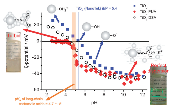
Figure 4. The titrimetric analysis of \zeta potential of the unmodified \text{TiO}_2 (NanoTek®) (blue filled square), \text{TiO}_2 -DSA (black circle), and \text{TiO}_2 -PUA (red filled diamond). The schematic illustration of the suggested dispersion mechanism and the images of the aqueous \text{TiO}_2 -PUA dispersion are also displayed.
