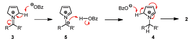
Scheme 2. Proposed Mechanism for Redox Isomerization
