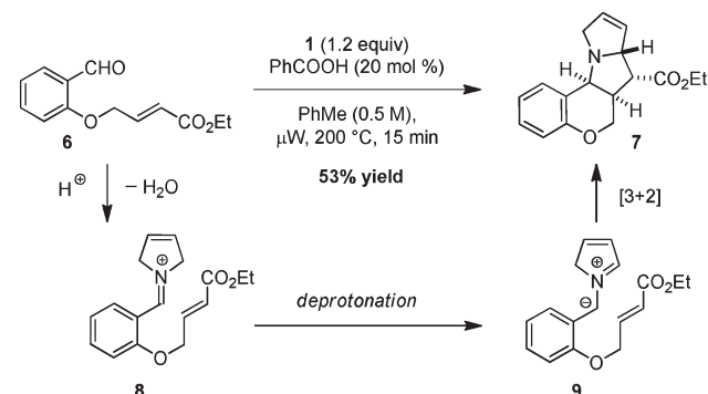
Scheme 3. Evidence for Azomethine Ylide Intermediates
