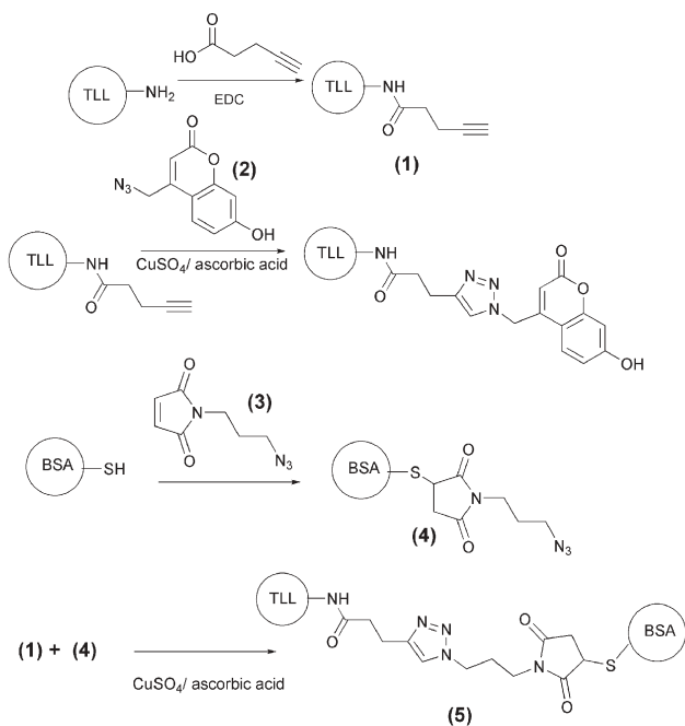
Scheme 1 Synthesis and characterization of the TLL-BSA hetero-dimer.
