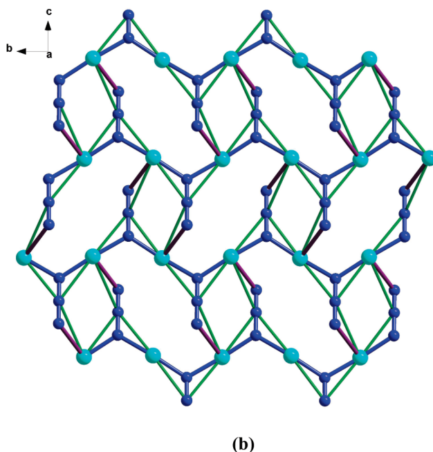
Figure 3. The 2D azido-copper net and topology for (a) 2 and (b) 3 . Blue bonds stand for equatorial coordination, the dark red for axial coordination, and the light green line for topology analysis.
