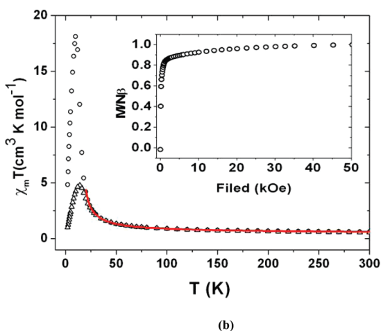
Figure 5. \chi_m T vs T plot at 0.2 T (circles) and 1.0 T (triangles). The solid line is the best fit to the experimental data. Inset: Magnetization vs field plot at 2.0 K for (a) 2 and (b) 3 .
