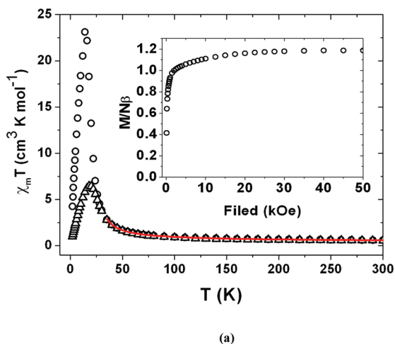
Figure 4. \chi_m T vs T plot for 1 at 0.3 T applied field. The solid line is the best fit to the experimental data. Inset: the plot of the field dependence of the magnetization at 2 K.
