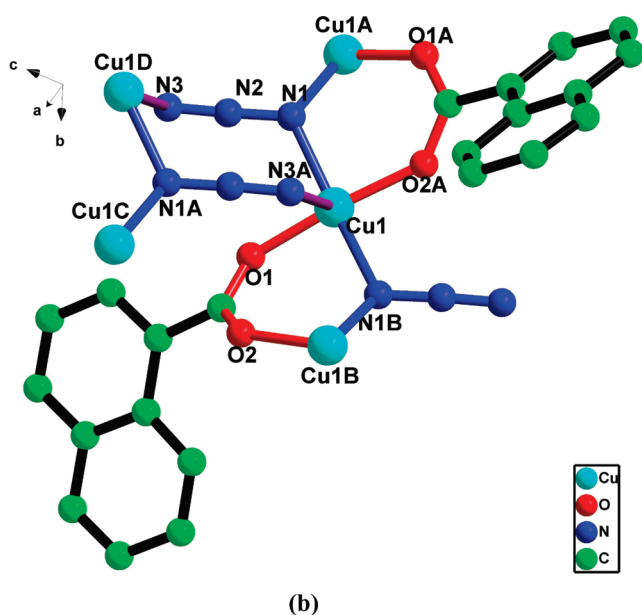
Figure 2. The linkage and coordination modes for complexes (a) 2 and (b) 3 . Blue bonds stand for equatorial coordination and the dark red for axial.
