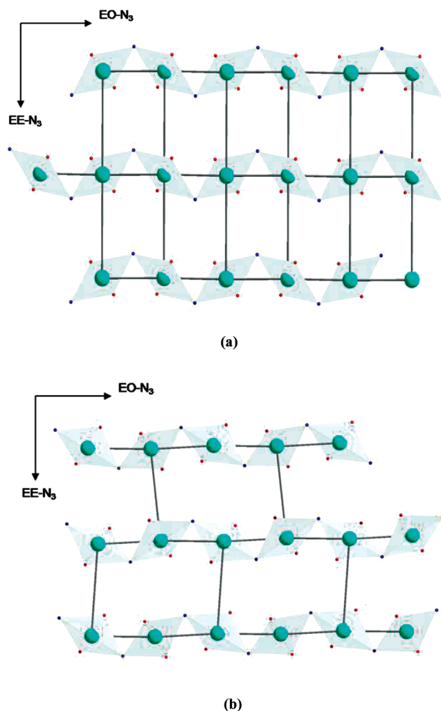
Figure 7. (a) View of 2 along the c direction of the unit cell (the \text{Cu}^{\text{II}} layers lay along the ab plane). The xy plane of the \text{Cu}^{\text{II}} centers are shown. (b) View of 3 along the a axis of the unit cell (the \text{Cu}^{\text{II}} layers lay along the bc plane). The xy planes on each \text{Cu}^{\text{II}} ion are shown.
