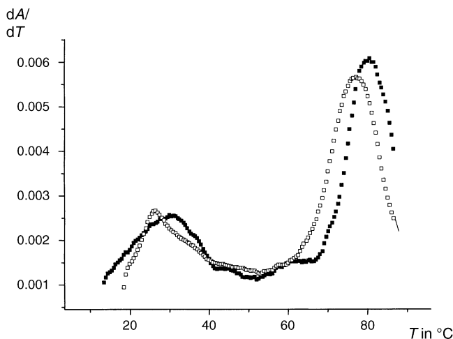
Figure 2. Plot of first derivative dA/dT versus temperature of the UV melting curves for the foldback triplex without (□) and with (■) \delta -carboline 7I .
