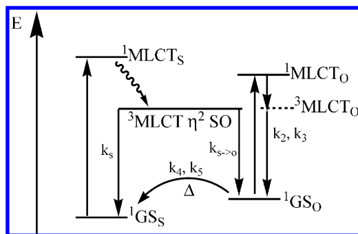
Figure 5. Modified Jablonski type diagram for [\text{Ru}(\text{bpy})_2(\text{OSOR})]^+ . ^1\text{GS}_\text{S} and ^1\text{GS}_\text{O} are the S-bonded and O-bonded ground states. ^1\text{MLCT}_\text{S} and ^1\text{MLCT}_\text{O} are S-bonded and O-bonded excited states. The O-bonded ^3\text{MLCT} state is denoted as a dashed line since the relative energy is not known.
