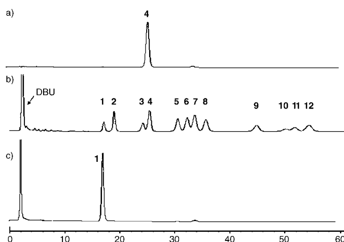
Figure 1. Amplification chromatogram using B(OH) 3 HPLC chromatogram (C18 column: 4.6 × 150 mm, eluted with a solution of water, acetonitrile, and methanol in a ratio of 52:18:30) of I(1,4,5)Bz 3 ( 4 ), b) DCL at 1.5 h after addition of DBU, and c) 72 h after addition of boric acid (94% of 1 ).
