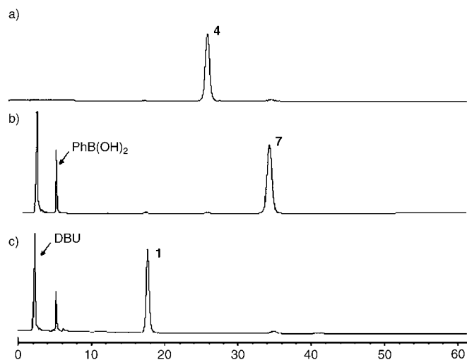
Figure 3. Direct migration chromatogram using \text{PhB(OH)}_2 a) The HPLC chromatogram of \text{I(1,4,5)Bz}_3 ( 4 ), b) 25 min after addition of DBU and \text{PhB(OH)}_2 (98 % of 7 ), c) after an additional 124 h (96 % of 1 ).
