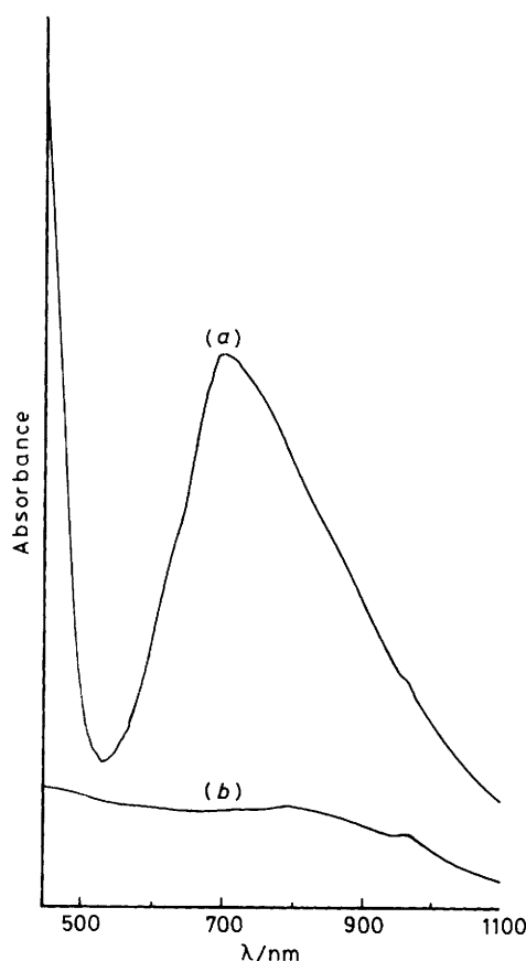
Figure 5. Electronic ( d-d ) spectra for (1) in \text{CH}_3\text{CN} ( 3 \times 10^{-4} \text{ mol dm}^{-3} , 0.1 \text{ mol dm}^{-3} [\text{NEt}_4][\text{ClO}_4] ), (a) before reduction; (b) after reduction
