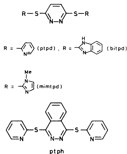
Figure 1. Structural formulae of the ligands ptpd, bitpd, mimtpd, and ptpd
