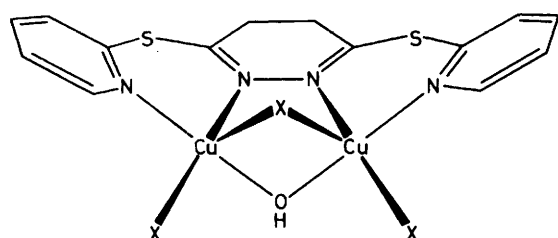
Figure 2. Structural representation of complexes (1) ( X = \text{Cl} ) and (2) ( X = \text{Br} )
