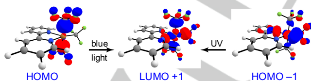
Figure 3. Both UV and blue light excite to the same \sigma^* orbital (LUMO + 1). This results in the formation of ^3\text{I} leading to CF 3 bond homolysis.
