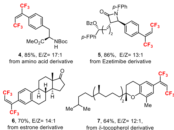
Scheme 2. Late-Stage 1,2-(Bis)trifluoromethylation of Bioactive Molecules a
