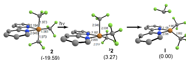
Figure 1. Computed geometries (uM06/LACVP**) and \Delta G_{\text{sol}} energies for 2 , 32 , and bpyCu(CF 3 ) 2 . Bond lengths are measured in angstroms (Å).
