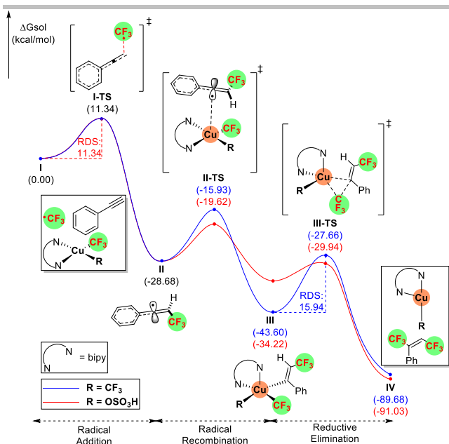
Figure 2. Computed \Delta G_{\text{sol}} energies (with uM06/cc-pVTZ(-f)-LACV3P**//uM06/LACVP**) for all intermediates and transition states along the reaction pathway from I to IV.
