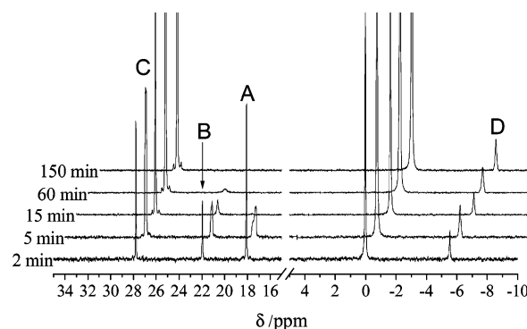
Figure 2. ^{31}\text{P} NMR of a catalytic benzaldehyde olefination with complex 7 at RT in CD 2 Cl 2 : (A) phosphorus ylide; (B) phosphazine XIII; (C) O=PPh 3 ; (D) PPh 3 .
