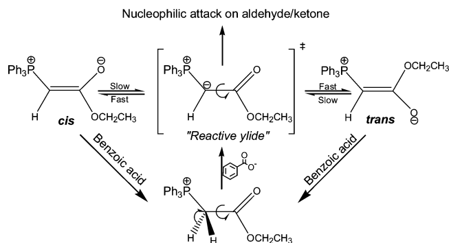
Scheme 4. "Activation" of Phosphorus Ylide by Benzoic Acid a
