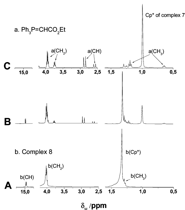
Figure 1. ^1\text{H} NMR of the reaction of complex 8 with PPh 3 in CD 2 Cl 2 at -30\text{ }^{\circ}\text{C} : (A) complex 8; (B) complex 8 after addition of less than 1 equiv of PPh 3 ; (C) complex 8 with 2.5 equiv of PPh 3 . The aromatic region is excluded for simplicity purposes.
