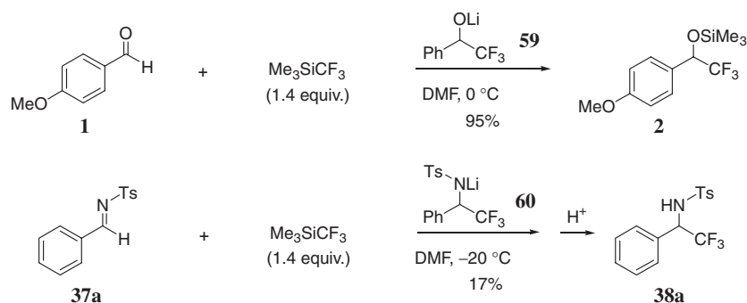
Scheme 2. Autocatalytic process.
