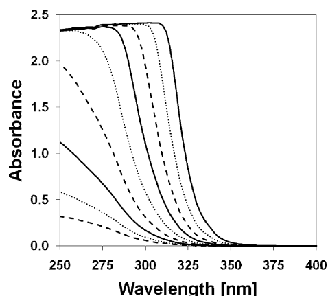
Figure 5. Absorption spectra of \text{Ti}_{17}\text{O}_{24}\text{OPr}_{20} ( \text{Ti}_{17} ) in \text{CH}_2\text{Cl}_2 at the following concentrations (right to left): 1.3, 0.63, 0.31, 0.16, 7.8 \times 10^{-2} , 3.9 \times 10^{-2} , 2.0 \times 10^{-2} , 9.8 \times 10^{-3} , and 4.9 \times 10^{-3} g/L.
