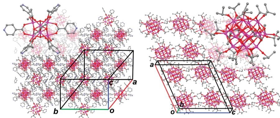
Figure 1. Periodic arrangement of the nanoclusters in crystals of (left) \text{Ti}_6\text{cat}_6 and (right) \text{Ti}_{17} , with the structures of individual molecules (insets). Ti, purple; O, red; C, gray; N, blue.
