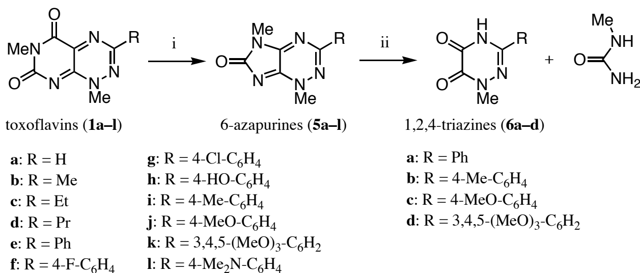
Scheme 2. Reagents and conditions: i, 10% aq NaOH, 5–25 °C, 1–3 d for R = H and alkyl, 60–70 °C, 10–45 min for R = aryl; ii, 10% NaOH in EtOH, reflux, 6 h.
