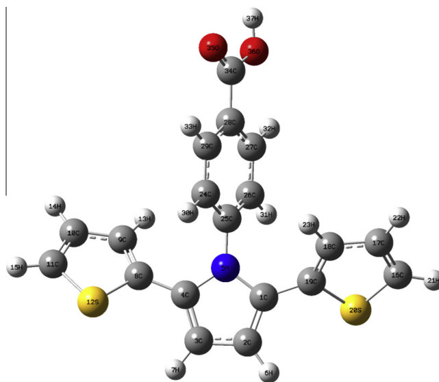
Fig. 2. Theoretical optimized geometric structure of the TPBA.
