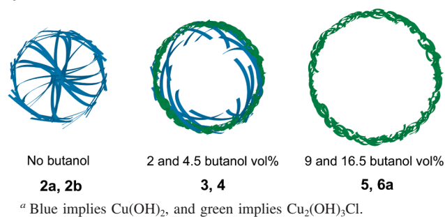
Scheme 2. Schematic Sectional View of the Different Morphologies and Sizes As a Function of the Butanol Volume Used in the Synthesis a
