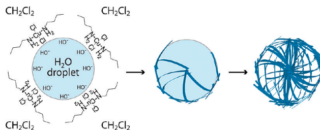
Scheme 1. CuCl 2 –Butylamine Complex Precipitation at the Water Droplet Surface and Anisotropic Growth of Cu(OH) 2
