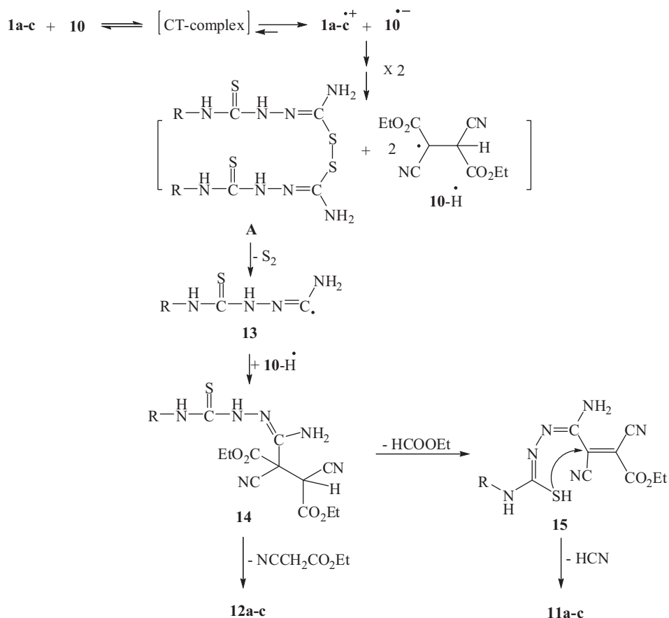
Scheme 4
