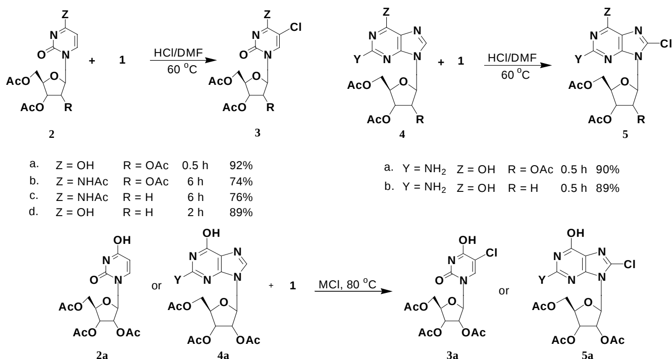
Scheme 1. Chlorination of Acetylated Nucleosides with 1
