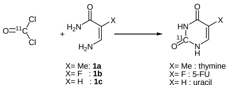
Scheme 1. Synthetic route of [2- ^{11}\text{C} ]pyrimidine derivatives.
