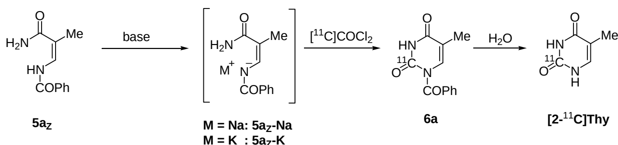
Scheme 8. Synthesis of [ 2\text{-}^{11}\text{C} ]Thy
