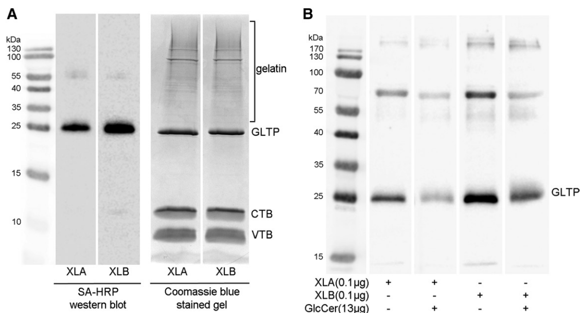
Fig. 4. XLA and XLB preferentially cross-links and shows substrate competition for GLTP. A: XLA or XLB (0.75 μM) was incubated with an equal mass of GLTP (2 mM), VTB, CTB, and gelatin. XLA and XLB were cross-linked to interacting proteins with UV light for 15 min. Western blot with SA-HRP shows GLTP was preferentially cross-linked, gel stained with Coomassie blue shows the presence of equal amounts of GLTP, VTB, CTB, and gelatin. B: GLTP, XLA, or XLB were incubated with or without GlcCer for 1 h at 37°C before cross-linking with UV light for 15 min. Representative Western blot with SA-HRP shows GlcCer reduces GLTP cross-linking for both XLA and XLB.
