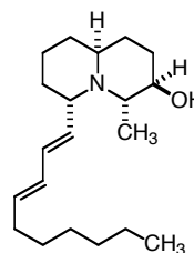
3 (Clavipictine B)
