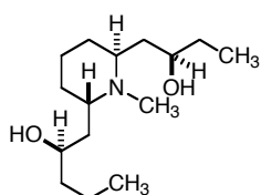
1 (Dihydroandrachne)
