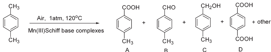
Scheme 1 The oxidation of p -xylene to PTA catalyzed by Mn(III) Schiff base complexes.
