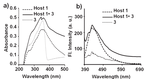
Figure 7. (a) Solid-state UV–visible absorption spectra of host 1 , host 1·3 complex, and coumarin. (b) Comparison of the solid-state fluorescence spectra of host 1 ( \lambda_{\text{exc}} = 358 nm), 3 ( \lambda_{\text{exc}} = 351 nm), host 1·3 complex ( \lambda_{\text{exc}} = 347 nm).
