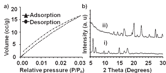
Figure 5. (a) CO_2 adsorption isotherm of host 1 at 273 K. (b) PXRD pattern of host 1 before (bottom) and after coumarin ( 3 ) absorption (top).
