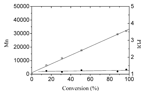
Figure 5. Polymerization of \epsilon -caprolactone initiated by complex 3 in toluene at 50\text{ }^{\circ}\text{C} . The relationship between the number-averaged molecular weight ( M_n ) and the conversion is shown.
