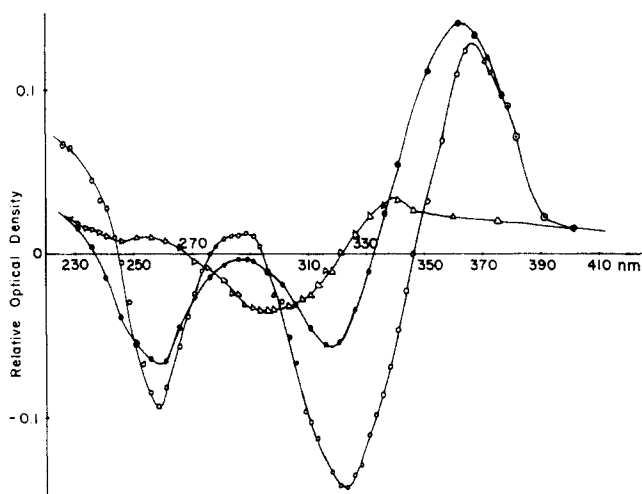
Figure 3. Short-lived transient absorption spectra (difference absorption spectra) at t = 0 (i.e., immediately after flash photolysis): trans -BPyE in n -hexane and in methanol (○); cis -BPyE in methanol (△).
