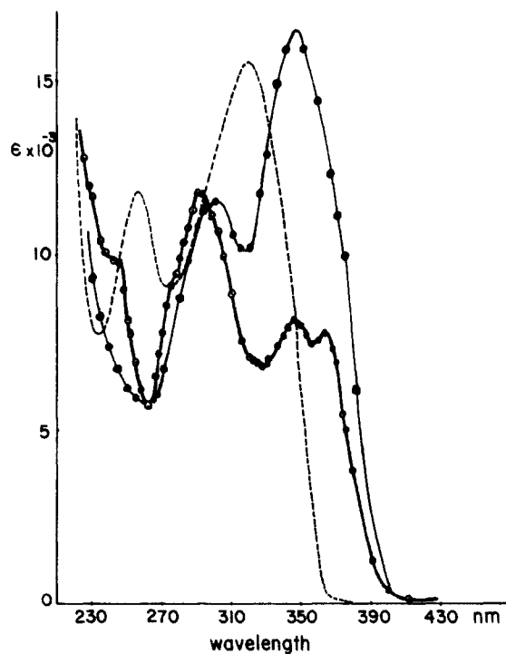
Figure 4. UV absorption (---) and triplet-triplet absorption spectra of trans -BPyE in n -hexane (●) and in methanol (○).
