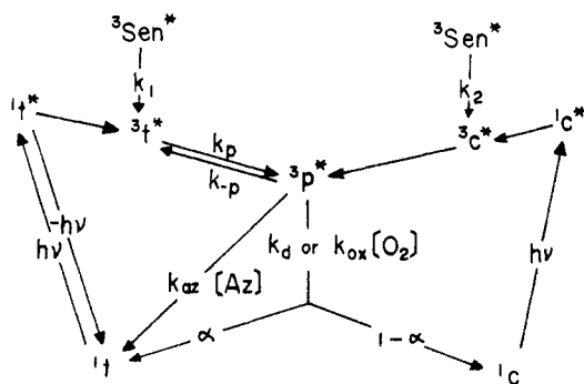
Scheme I. Mechanism of the Photoisomerization of BPyE (Triplet Decay) and Interaction with Quenchers, where ^3p^* is the Twisted (Phantom) Triplet Excited State
