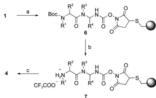
Scheme 2. Polymer-assisted synthesis of 1,3,5-triazepan-2,6-diones 4 . a) (i) DPPA (1.1 equiv), Et 3 N (1.1 equiv), RT, 30 min; (ii) 70 °C for 1.5 h; (iii) PS-HOSu (0.3 equiv), 70 °C, 40 min; b) TFA/CH 2 Cl 2 (1:1), 2 × 5 min, RT, washings; c) DIPEA (1.1 equiv), 40–60 °C, 4 × 30 min.
