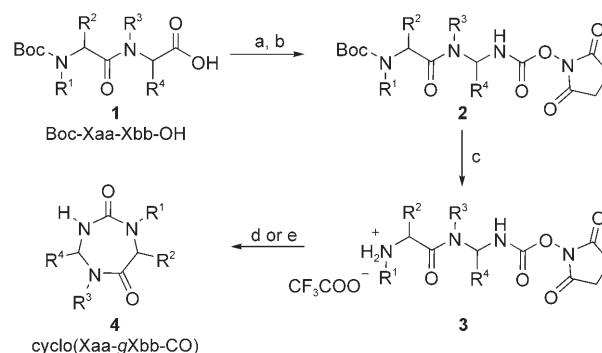
Scheme 1. Solution-phase synthesis of 1,3,5-triazepan-2,6-diones 4 . a) EtOCCl, NMM, THF, -20^{\circ}\text{C} , then \text{NaN}_3 in \text{H}_2\text{O} ; b) toluene, 65^{\circ}\text{C} , then HOSu, py; c) TFA, 30 min; d) DIEPA, MeCN; e) PS-DIPEA, \text{CH}_2\text{Cl}_2 .
