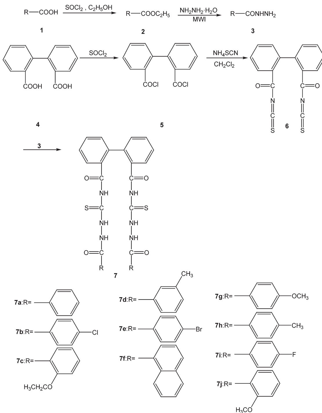
Scheme 1 The synthetic route of molecular tweezers 7a–j .
