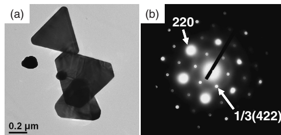
Figure 2. (a) A transmission electron micrograph of Au nanosheets synthesized by using reducing stabilizer 1 ·2HCl and (b) its electron diffraction pattern.
