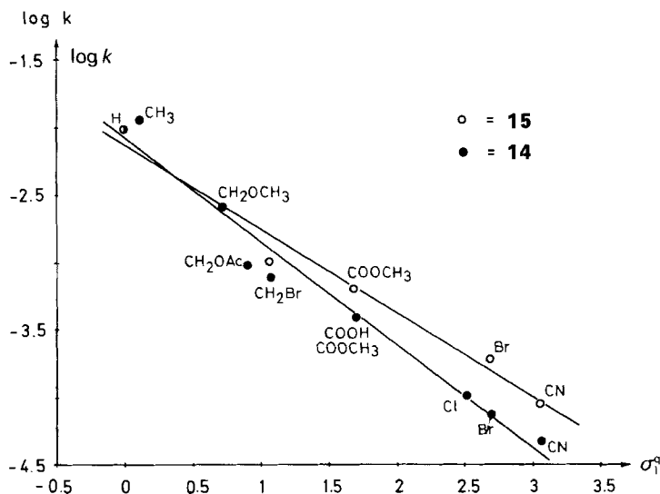
Fig. 1. Plots of \log k for 10^{-3} M solutions of 4 c -substituted 2 c - ( 14 ) and 2 a -adamantyl p-nitrobenzenesulfonates 15 in 80% (v/v) EtOH against inductive substituent constants \sigma_i^q
