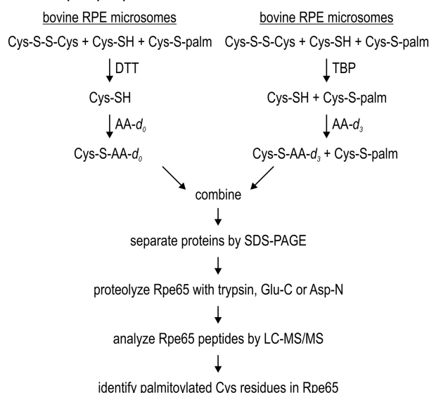
FIGURE 4. Strategy to determine palmitoylation status of Cys residues in Rpe65. A, flow chart for the preparation of Rpe65 peptide samples for LC-MS analysis. One aliquot of bovine RPE membranes is incubated with DTT, which reduces disulfides and de-palmitoylates Cys residues in all proteins, including Rpe65. The resulting free sulfhydryl groups are alkylated by incubating with nondeuterated acrylamide (AA- d_0 ). A second aliquot is incubated with TBP to reduce disulfide without de-palmitoylating Cys residues. Next, the nonpalmitoylated sulfhydryls are alkylated by incubating with triple-deuterated acrylamide (AA- d_3 ). These two aliquots are pooled and the constituent proteins separated by SDS-PAGE. The Rpe65 band is excised and digested with trypsin, endopeptidase Glu-C, and/or Asp-N, and the resulting peptides are analyzed by LC-MS/MS. B, diagram showing predicted spectral patterns for the different potential palmitoylation states of a Cys residue. If a Cys-containing peptide is not palmitoylated, it would incorporate equal amounts of AA- d_0 and AA- d_3 . Therefore, the two sets of native isotopic peaks that differ by three atomic mass units would be equally abundant in the spectrum. If the Cys residue is partially palmitoylated, the triple-deuterated ions would be correspondingly less abundant than the nondeuterated ions. If the Cys residue is fully palmitoylated, no triple-deuterated ions would be present in the spectrum.
