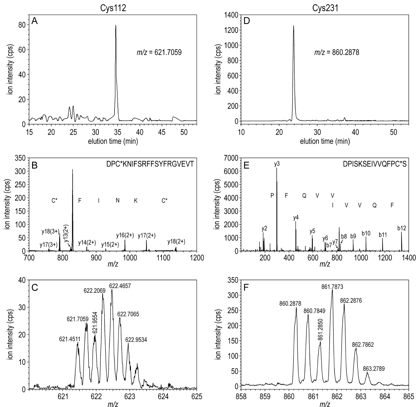
FIGURE 3. ESI-MS/MS data showing similar abundance of AA- d_0 - and AA- d_3 -modified peptides containing residues Cys-112 and Cys-231. A, selected ion monitoring chromatogram of an ion with m/z 621.7059. This ion corresponds to tetra-charged Asp-N peptide AN110–129 from bovine Rpe65 after modification of Cys-112 with AA- d_0 . B, tandem mass spectrum of the 621.7059 m/z ion with the corresponding observed b- and y-ions indicated. C, zoom spectrum of the indicated m/z values acquired at 35 min. Note the deviation from the ideal d_0/d_3 distribution shown on Fig. 4 due to the overlap of native isotopic d_0 ions on the d_3 ion species. The similar abundance of the corresponding AA- d_0 and AA- d_3 -labeled ions indicates that Cys-112 is not palmitoylated. D, selected ion monitoring chromatogram of an ion with m/z 860.2878 corresponding to the double-charged Asp-N peptide AN218–232 from bovine Rpe65 after modification of Cys-231 with AA- d_0 . E, tandem MS chromatogram of the m/z 860.2878 ion with the corresponding b- and y-ions indicated. F, zoom spectrum of the indicated m/z values acquired at 24 min. The similar abundances of the corresponding AA- d_0 - and AA- d_3 -labeled ions indicate that Cys-231 is not palmitoylated. Note that the b- and y-ions containing Cys residues show similar d_0/d_3 doublet peaks, whereas ions lacking Cys show only singlet peaks.
