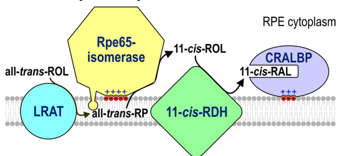
FIGURE 10. A, electrostatic surface potential of bovine Rpe65. Regions with negative electrostatic potential (acidic) are shown in red, neutral regions are shown in white, and regions with positive electrostatic potential (basic) are shown in blue. The left and right images are from opposite sides of the protein. Note the strongly basic (blue) regions, corresponding to residues 294–298, 354–359, and other basic residues scattered throughout the sequence. B, hypothesized interactions of visual cycle proteins on the ER membrane of an RPE cell. Lecithin:retinol acyltransferase (LRAT) and 11- cis -RDH are integral-membrane proteins, whereas both Rpe65 and CRALBP (40) are soluble proteins with affinity for acidic phospholipid headgroups. Following synthesis by lecithin:retinol acyltransferase, Rpe65 extracts all- trans -RP from the membrane and isomerizes it to 11- cis -ROL. 11- cis -RDH oxidizes it to 11- cis -RAL, which binds to CRALBP and is transferred to the apical plasma membrane of the RPE cell for export to the photoreceptors.
