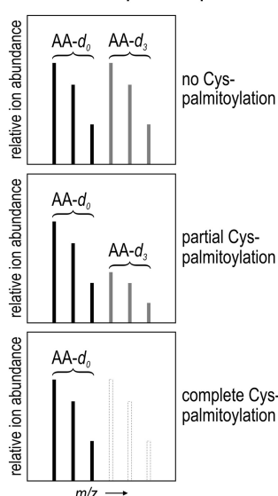
FIGURE 4. Strategy to determine palmitoylation status of Cys residues in Rpe65. A, flow chart for the preparation of Rpe65 peptide samples for LC-MS analysis. One aliquot of bovine RPE membranes is incubated with DTT, which reduces disulfides and de-palmitoylates Cys residues in all proteins, including Rpe65. The resulting free sulfhydryl groups are alkylated by incubating with nondeuterated acrylamide (AA- d_0 ). A second aliquot is incubated with TBP to reduce disulfide without de-palmitoylating Cys residues. Next, the nonpalmitoylated sulfhydryls are alkylated by incubating with triple-deuterated acrylamide (AA- d_3 ). These two aliquots are pooled and the constituent proteins separated by SDS-PAGE. The Rpe65 band is excised and digested with trypsin, endopeptidase Glu-C, and/or Asp-N, and the resulting peptides are analyzed by LC-MS/MS. B, diagram showing predicted spectral patterns for the different potential palmitoylation states of a Cys residue. If a Cys-containing peptide is not palmitoylated, it would incorporate equal amounts of AA- d_0 and AA- d_3 . Therefore, the two sets of native isotopic peaks that differ by three atomic mass units would be equally abundant in the spectrum. If the Cys residue is partially palmitoylated, the triple-deuterated ions would be correspondingly less abundant than the nondeuterated ions. If the Cys residue is fully palmitoylated, no triple-deuterated ions would be present in the spectrum.
