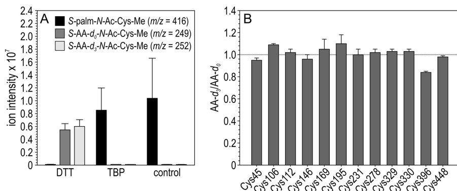
FIGURE 5. Analysis of Rpe65 S-palmitoylation. A, effects of DTT and TBP on Cys palmitoylation. S-Palm-N-Ac-Cys-Me was treated with DTT, TBP, or without a reducing agent (control) followed by reaction with a 1:1 mixture of AA- d_0/d_3 . This histogram shows the ion intensities of S-palm-N-Ac-Cys-Me ( m/z = 416 ), S-AA- d_0 -N-Ac-Cys-Me ( m/z = 249 ), and S-AA- d_3 -N-Ac-Cys-Me ( m/z = 252 ) in the different samples. Note the virtual absence of palmitoylated-Cys in the sample incubated with DTT and the presence of only palmitoylated Cys in the samples incubated with TBP or no reducing agent (control). B, AA- d_3/d_0 ratio for each Cys residue in bovine Rpe65. This ratio is equivalent to the fraction of nonpalmitoylated Cys in each peptide. The values were normalized to the peptide containing Cys-231, which is known to be nonpalmitoylated. Except for Cys-396, the other 11 Cys residues show AA- d_3/d_0 values close to 1, indicating nonpalmitoylation of these residues in bovine Rpe65. Error bars show standard deviations ( n = 3 ).
