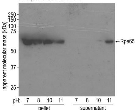
FIGURE 8. Rpe65 dissociates from microsomal membranes at high pH. Bovine RPE microsomes were incubated in buffers at the indicated pH values and then disrupted by nitrogen cavitation. After centrifugation, the resulting high speed pellets and supernatants were separated by SDS-PAGE. A, Coomassie-stained gel of the pellet and supernatant fractions. B, Rpe65 immunoblot of the same fractions. Note the release of Rpe65 from membranes into the supernatant between pH 10 and 11.
