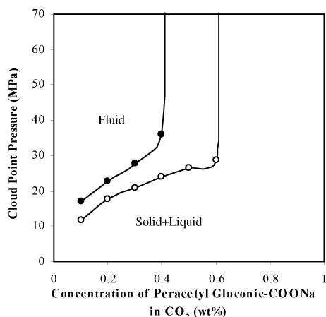
Figure 3. Phase behavior of peracetyl gluconic-COONa/CO 2 mixtures at 40 °C. W = 0 (○); W = 10 (●).
