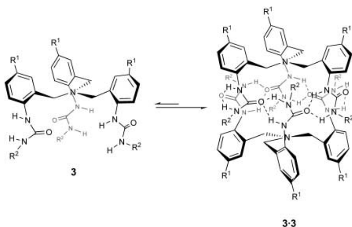
Scheme 3. Self-association of tris(ureas) 3 in solution of noncompetitive hydrogen-bonding solvents.
