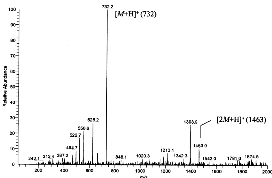
Figure 7. ESI mass spectrum of a \text{CHCl}_3 solution of 3a .
