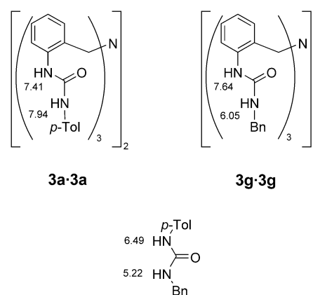
Scheme 4. Chemical shifts ( \text{CDCl}_3 ) for the NH resonances in 3a·3a and 3g·3g compared to a reference urea.
