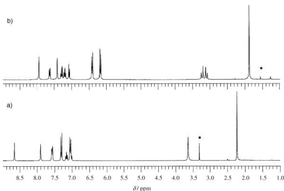
Figure 5. ^1\text{H} NMR spectra (300 MHz) of 3a a) in [\text{D}_6]\text{DMSO} and b) in \text{CDCl}_3 at 296 K; asterisks label the signals for residual water.
