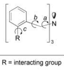
Figure 1. Tribenzylamine functionalized at the 2-position. Letters a , b , and c represent the bond rotations which would be restricted in a tripod–tripod assembly.
