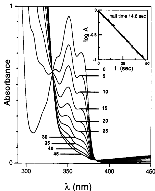
Figure 1. UV-vis spectra of the reaction products from photolysis of 2-iodo-4-[3-(trifluoromethyl)-3 H -diazirin-3-yl]benzyl acetate ( 10 ). A solution (2 mM) in cyclohexane was irradiated with filtered UV light ( \lambda > 320 nm) for increasing periods of time (in seconds) as indicated with numbers. The spectra show the decay of the diazirine characteristic absorption with a maximum at 351 nm. The inset shows the decay as a function of time of photolysis in a semilogarithmic plot.
