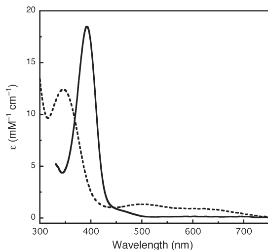
Figure 1. UV-vis spectra of the [(\text{TMED})_2\text{Cu}(\text{III})_2(\mu_2\text{-O})_2]^{2+} species (solid, [\text{Cu}] = 1 \text{ mM} , \text{CF}_3\text{SO}_3^- , acetone) and proposed [(\text{TMED})_3\text{Cu}(\text{III})\text{Cu}(\text{II})_2(\mu_3\text{-O})_2]^{3+} (dash, [\text{Cu}] = 1 \text{ mM} , \text{CF}_3\text{SO}_3^- , THF) at 183 K.
