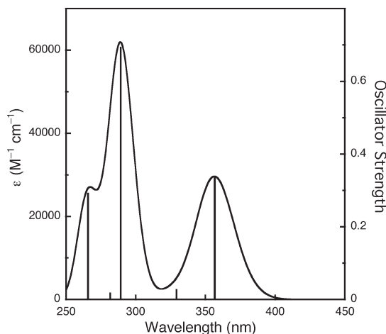
Figure 6. Oscillator strength and simulated electronic spectra of [(\text{TMED})_2\text{Cu}(\text{III})_2(\mu_2\text{-O})_2]^{2+} from DFT calculation with PCM-TD-B3LYP/BS1//B3LYP/6-31G(d) method ( \text{FWHM} = 2500 \text{ cm}^{-1} ).
