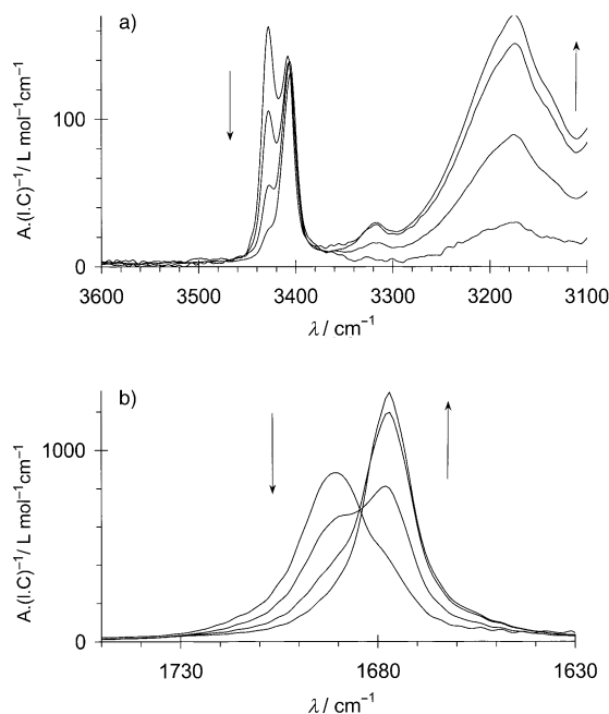
Figure 7. Normalized FTIR spectra of solutions of DIPPU in carbon tetrachloride versus concentration ( 10^{-4} , 10^{-3} , 10^{-2} , and 10^{-1} mol L ^{-1} ). Spectral regions characteristic of a) N–H and b) C=O. Arrows indicate the direction of change with increasing concentration.
