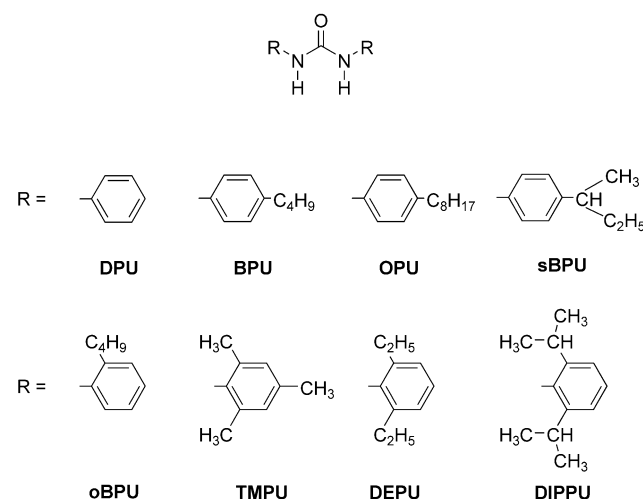
Scheme 6. Structures of N,N' -diarylureas studied.
