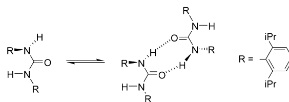
Scheme 7. Proposed association pattern for DIPPU .
