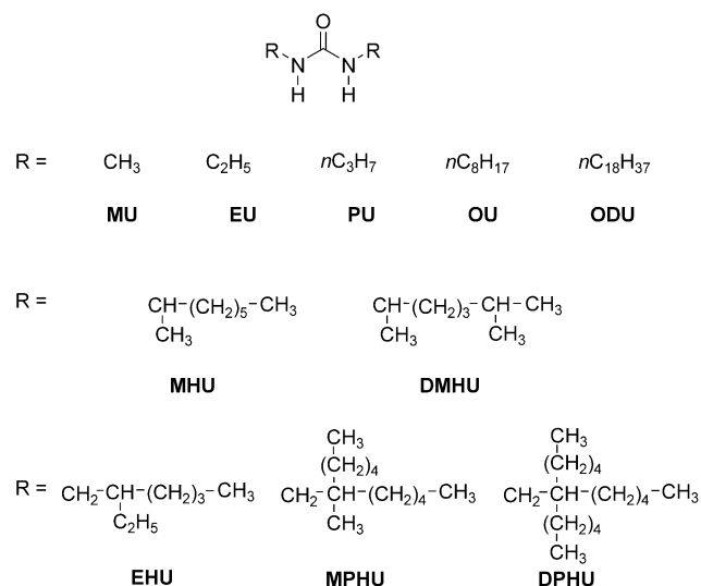
Scheme 2. Structures of N,N' -dialkylureas studied.
