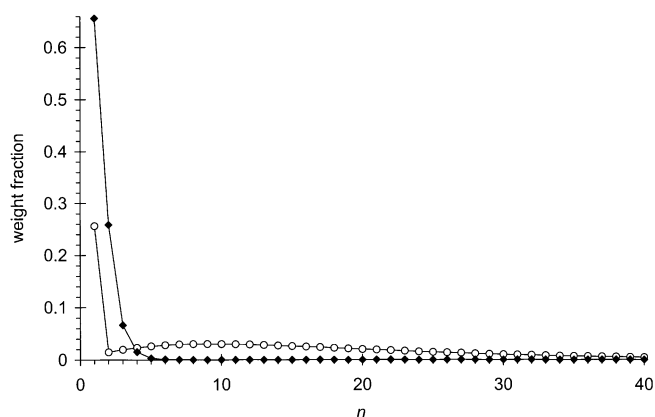
Figure 4. Calculated n -mer distribution in a 10^{-2} mol L ^{-1} solution of EHU (○) and DPHU (◆). (The values of the constants used are in Table 2.)
