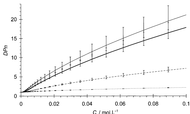
Figure 5. Calculated number-average degree of polymerization versus concentration, in a solution of EU (—), EHU (— — —), MPHU (---), and DPHU (····). (The values of the constants used are in Table 2.)
