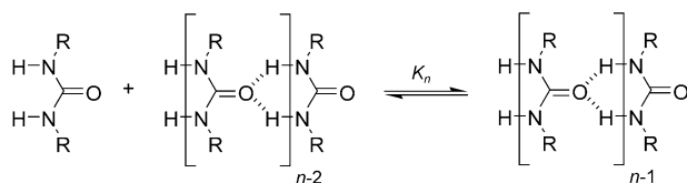
Scheme 5. Definition of the association constant K_n , n \geq 2 .
