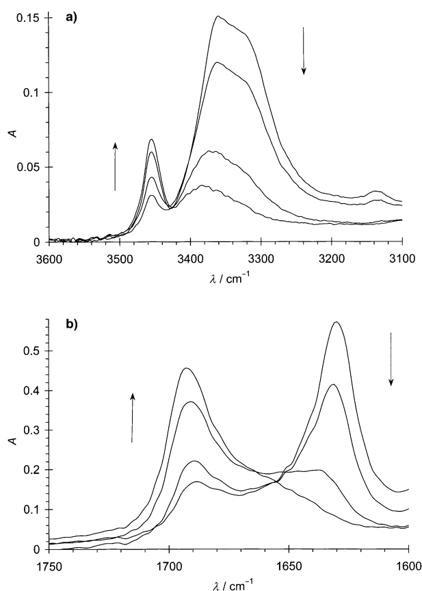
Figure 2. FTIR spectra of a 2.34 g L -1 ( 10^{-2} mol L -1 ) solution of EHU in carbon tetrachloride versus temperature (15, 30, 45, and 60 °C). Spectral regions characteristic of a) N–H and b) C=O. Arrows indicate the direction of change with increasing temperature.
