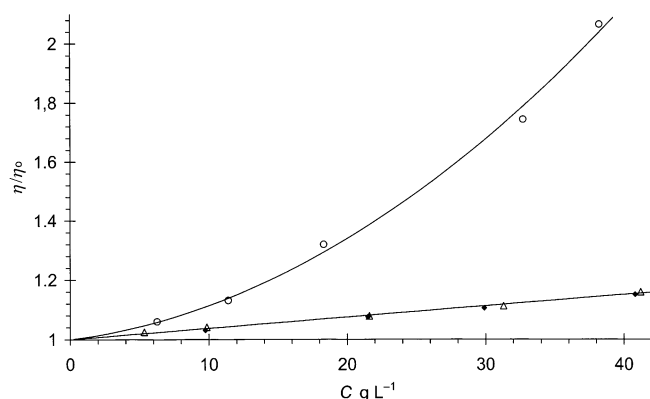
Figure 6. Relative viscosity of EHU (○), DIPPU (△) and DPHU (◆) versus concentration in carbon tetrachloride at 25 °C.
