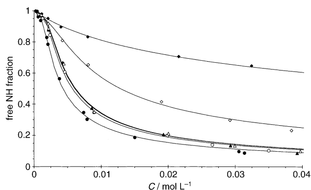
Figure 3. Fraction of free NH groups of EU (●), EHU (○), MHU (▲), DMHU (△), MPHU (◇), and DPHU (◆) versus concentration in carbon tetrachloride at room temperature. The curves are calculated according to ref. [16], with the constants reported in Table 2.
