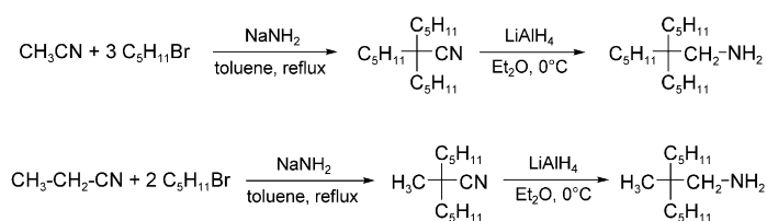
Scheme 4. Synthesis of two primary amines.
