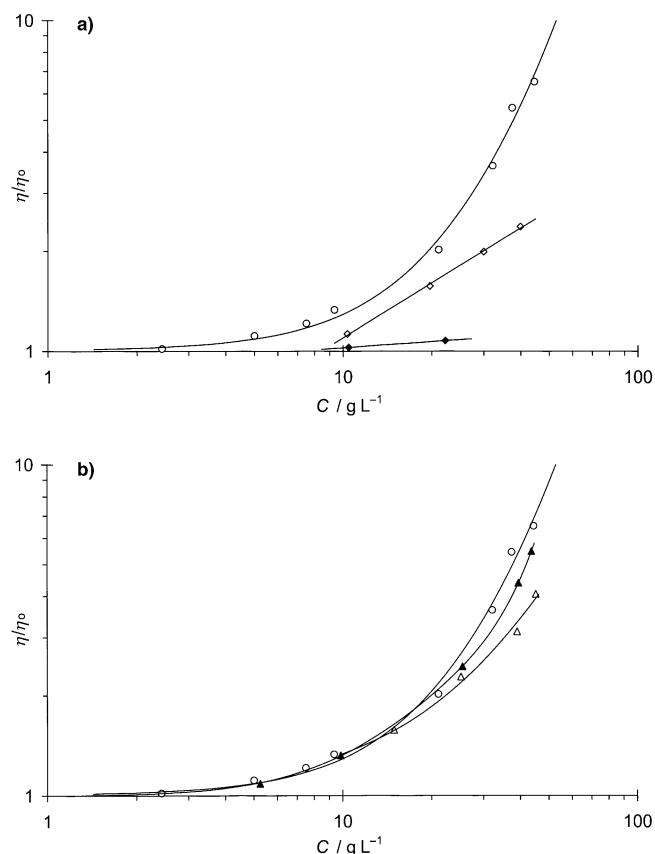
Figure 1. Relative viscosity of a) EHU (○), MPHU (◇) and DPHU (◆) and b) EHU (○), MHU (▲) and DMHU (△) versus concentration in heptane at 25 °C. The curves are a guide for the eye only.
